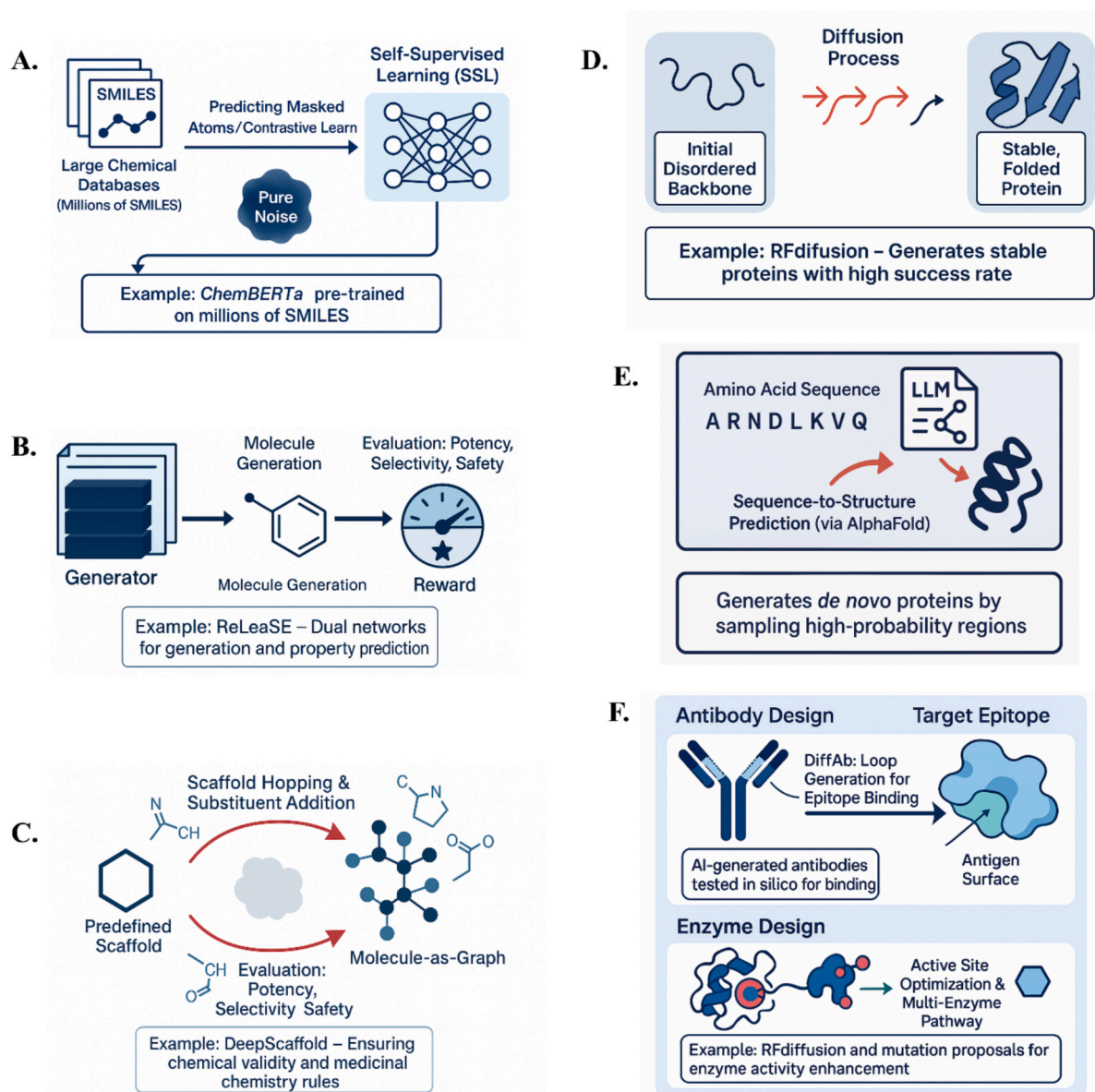
Fig. 2. Generative AI strategies for molecular and protein design. (A–C) Approaches for small molecule optimization using self-supervised learning (ChemBERTa), reinforcement learning (ReLeaSE), and graph-based models (DeepScaffold). (D–F) Protein design methods, including diffusion models (RFdiffusion), large language models for sequence generation, and applications in antibody and enzyme engineering.
