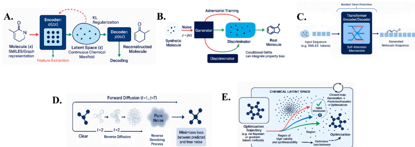
Fig. 1. Architectures of deep generative models and latent space optimization in molecular design. (A) Variational Autoencoders (VAEs), (B) Generative Adversarial Networks (GANs), (C) Transformer-based models, and (D) Denoising Diffusion Models generate molecules using distinct mechanisms. (E) Latent space optimization explores continuous chemical manifolds to design molecules with desired properties.
